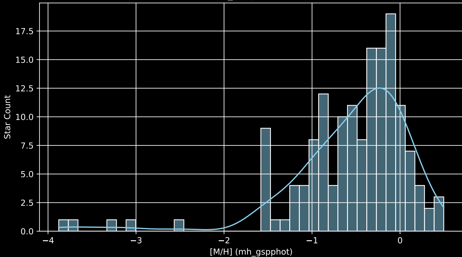
APOGEE DR17 Field: [000-17-C [M/H] (mh_gspphot) (n= 155)
