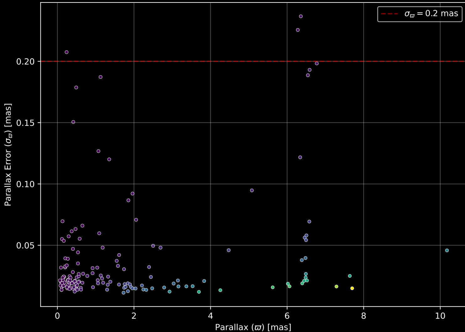
APOGEE DR17 Field: [000-17-C] Parallax Quality (n= 156)
