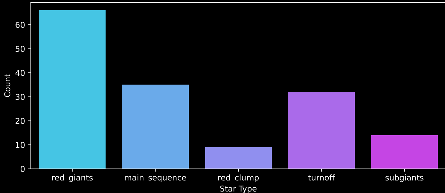
APOGEE DR17 Field: [000-17-C] Count plot of Star Type
