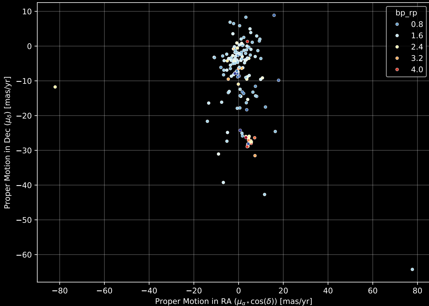
APOGEE DR17 Field: [000-17-C] Proper Motion Diagram (n= 156)
