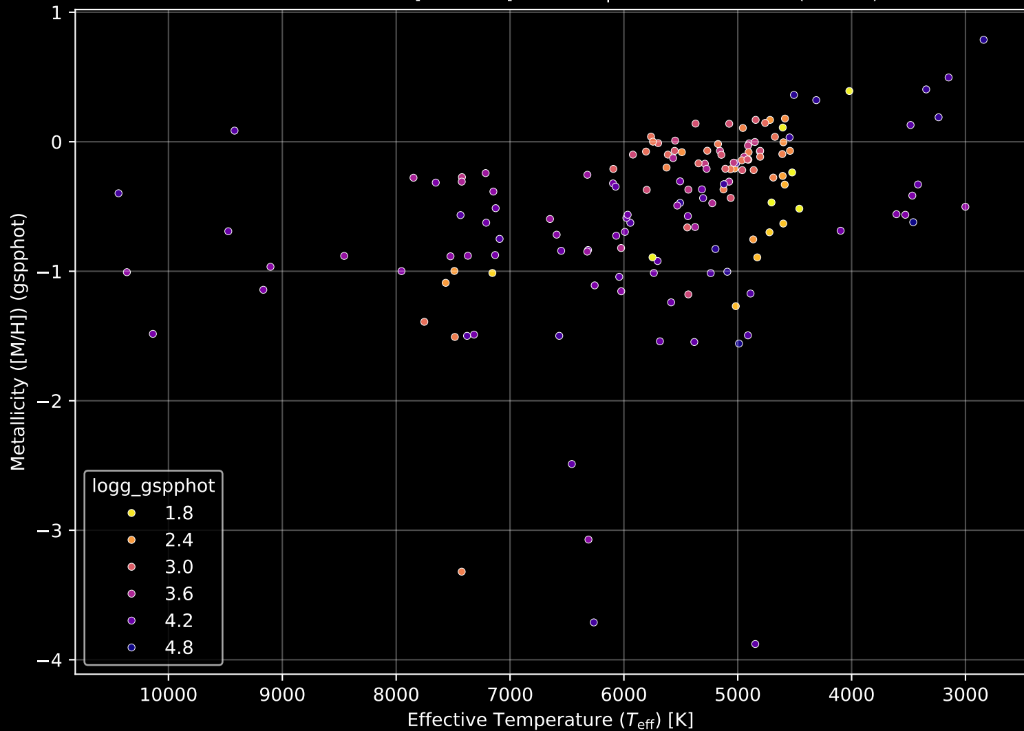
APOGEE DR17 Field: [000-17-C] Stellar Population Parameters (n= 156)
