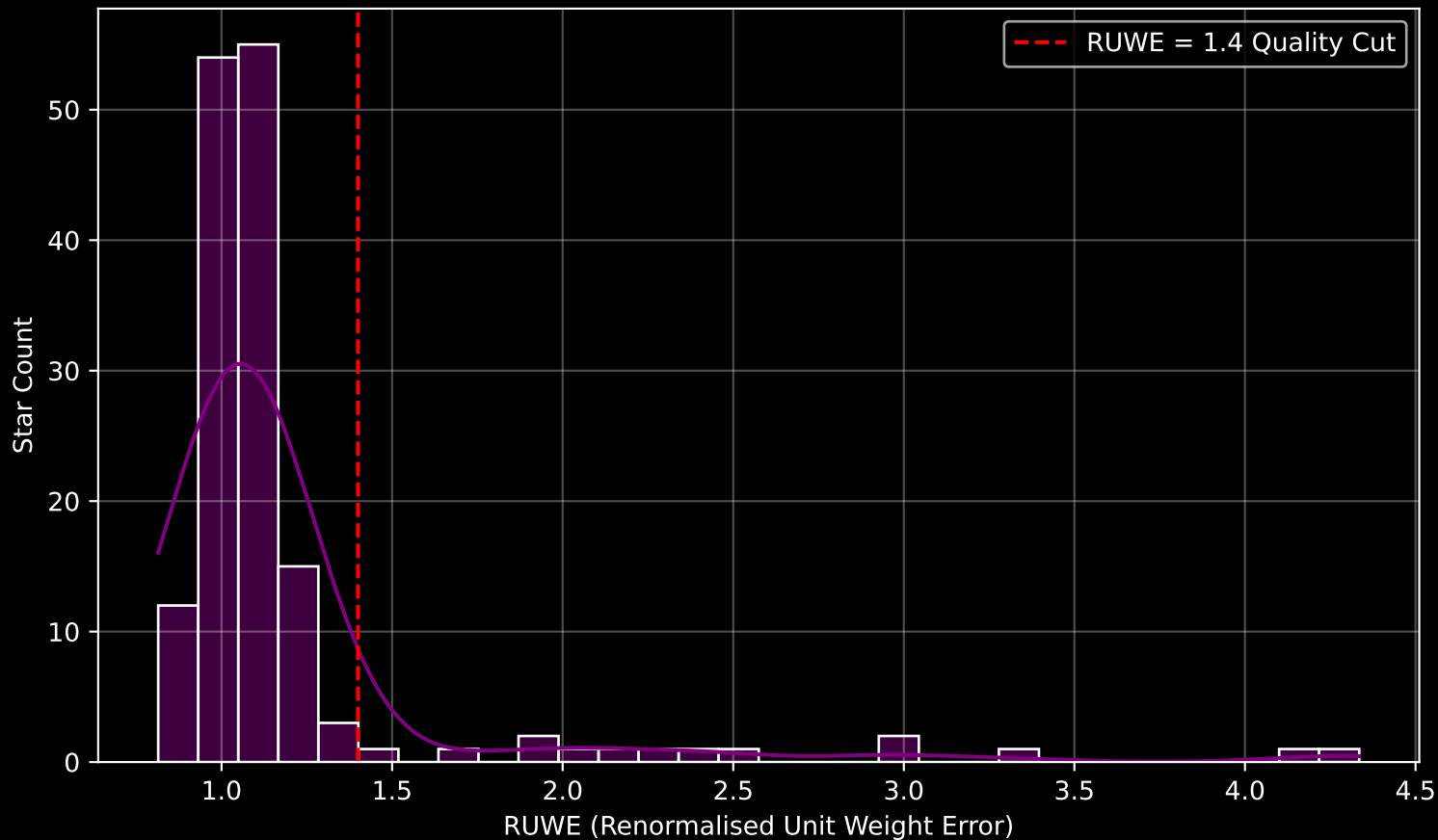
GAPOGEE DR17 Field [000-17-C] RUWE Distribution (n= 153)
