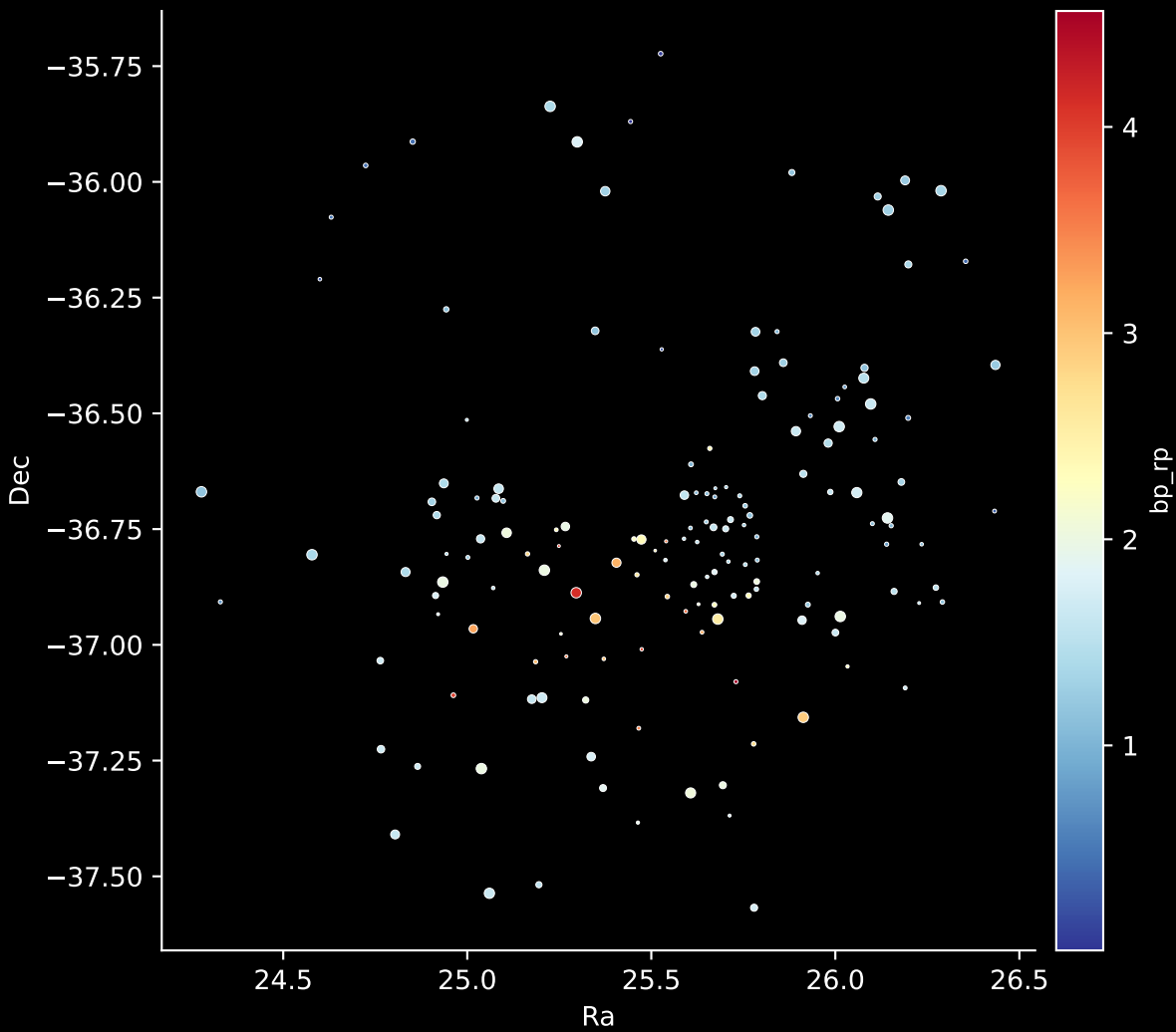
APOGEE DR17 Field: [000-17-C] Stars: 156
